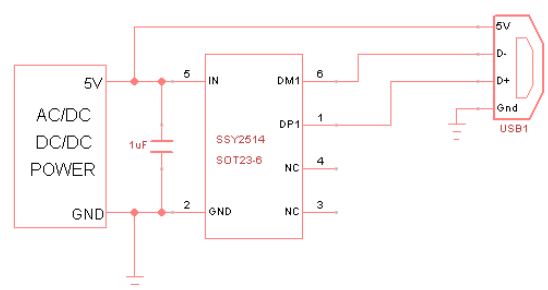
1×12W Application (SSY2514)
