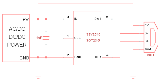
Apple 2.4A Application (SSY2515)
