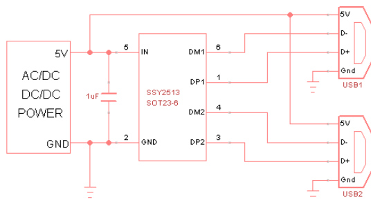
2×12W Application (SSY2513)
