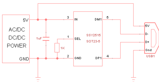
Apple 1A Application (SSY2515)
