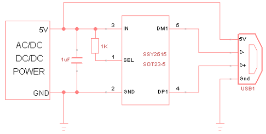
Apple 2A Application (SSY2515)
