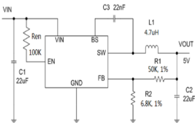
Figure 1. Basic Application Circuit for VOUT=5V
